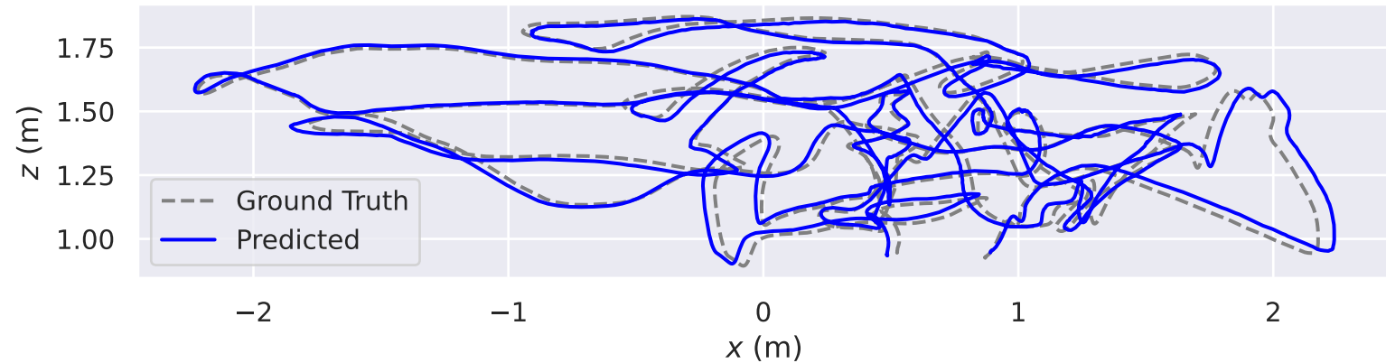
Euroc V1_01_easy Trial #1 (ATE: 0.217)
