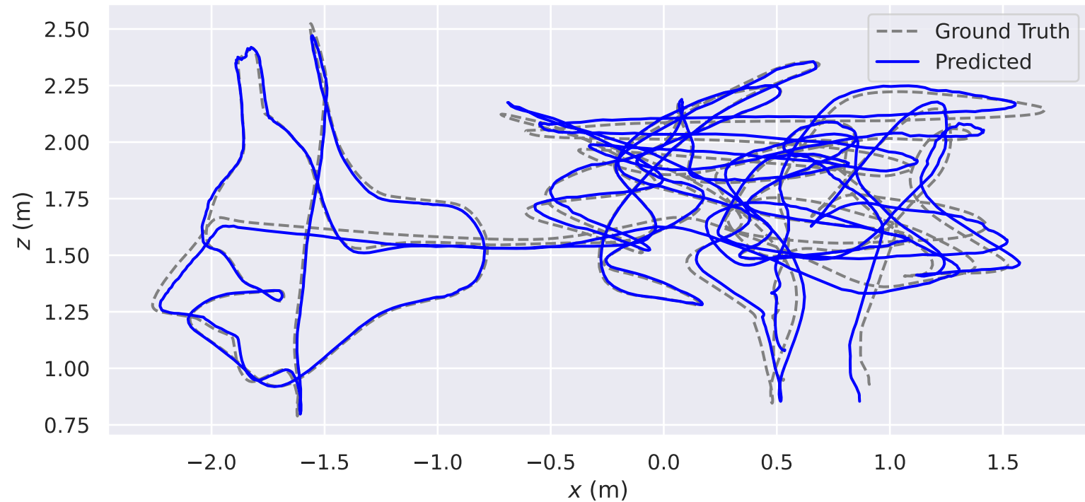
Euroc V1_03_difficult Trial #1 (ATE: 0.229)
