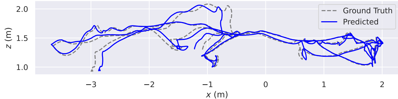
Euroc V2_01_easy Trial #1 (ATE: 0.235)
