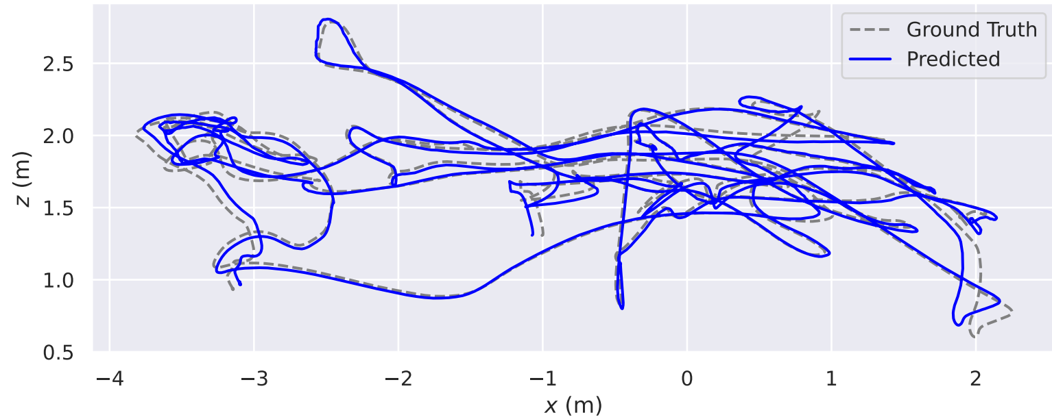
Euroc V2_02_medium Trial #1 (ATE: 0.082)
