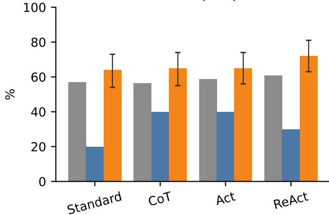
FEVER (Acc)
