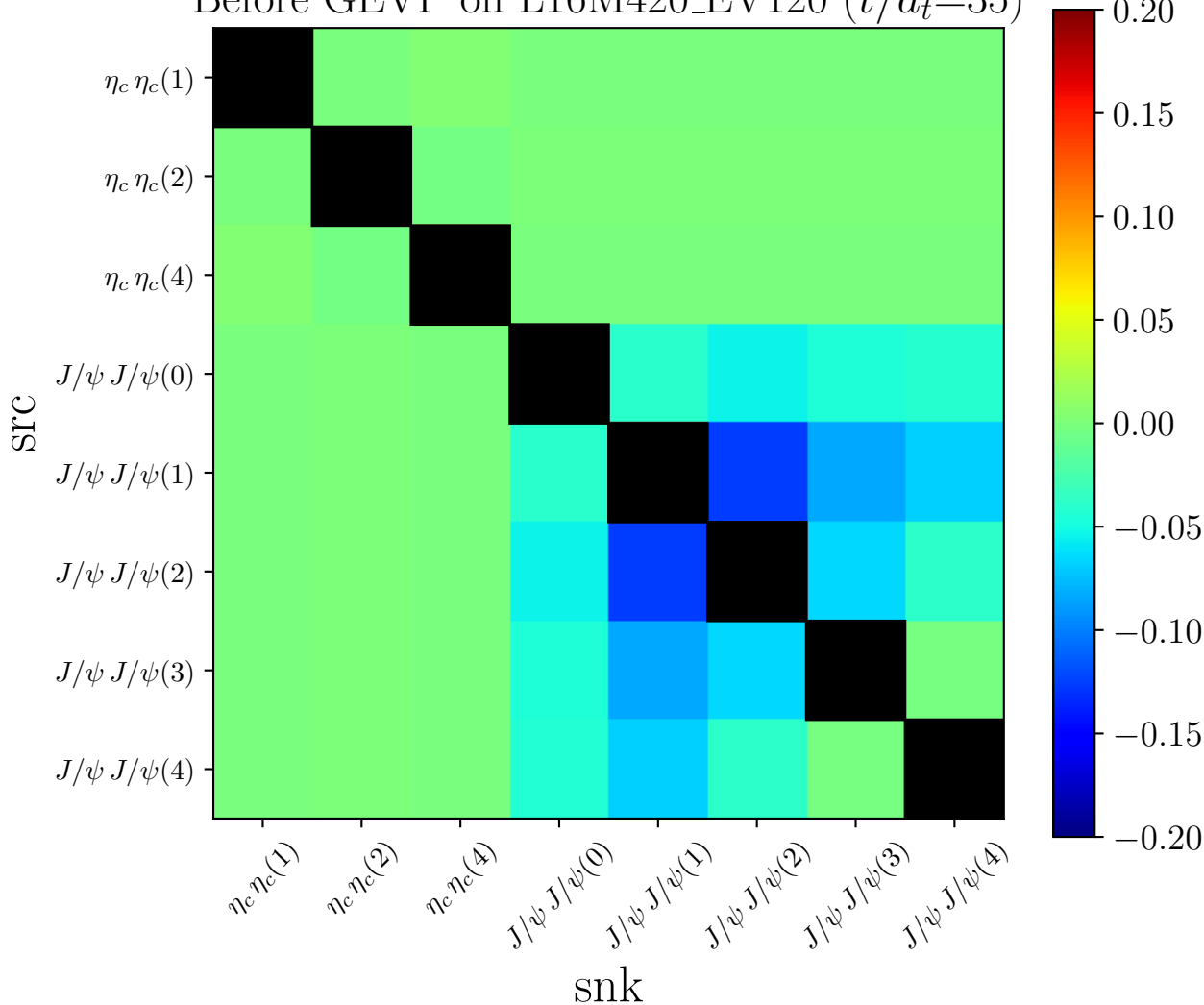
Before GEVP on L16M420_EV120 ( t/a_t=35 )
