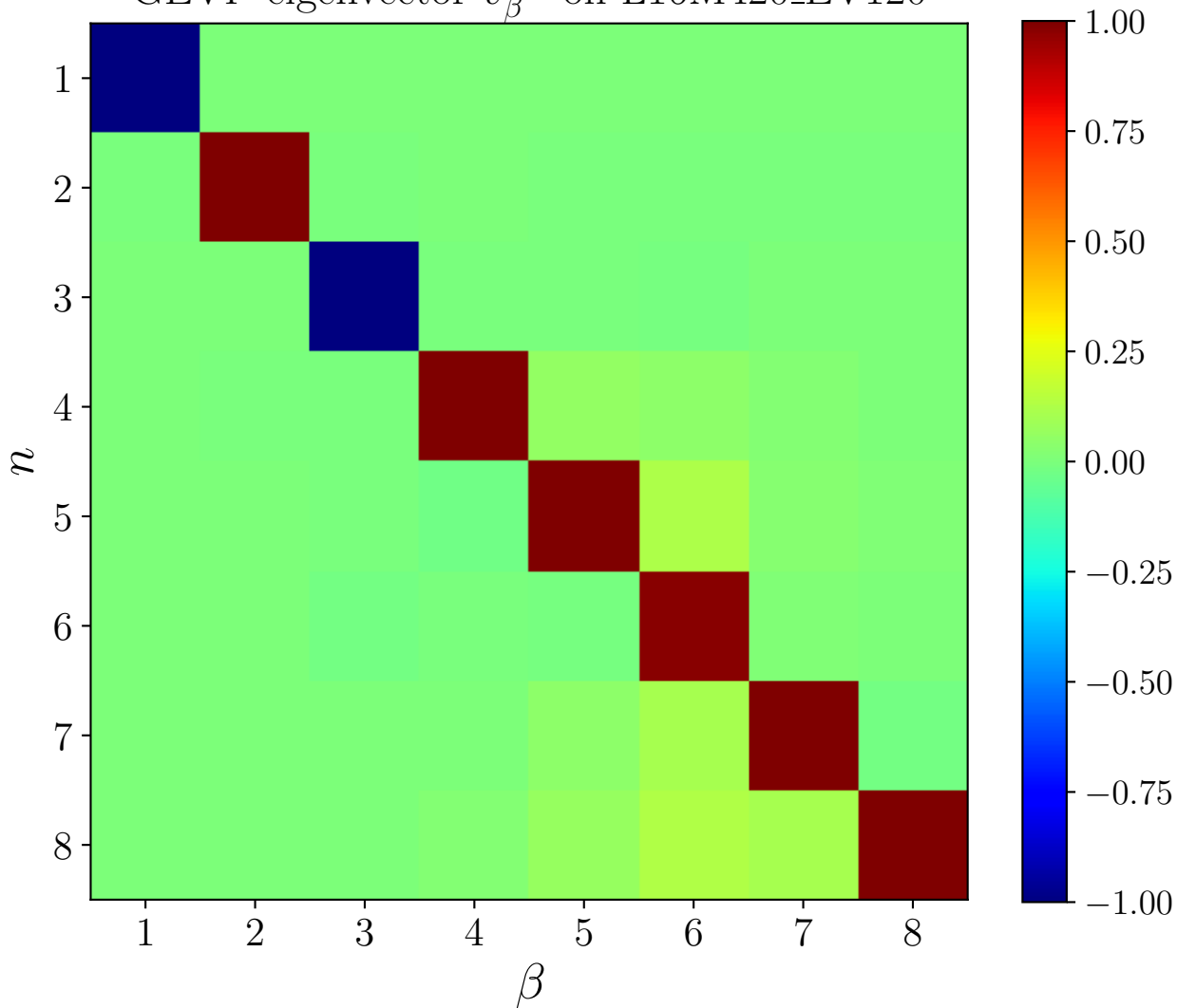
GEVP eigenvector v_{\beta}^{(n)} on L16M420_EV120
