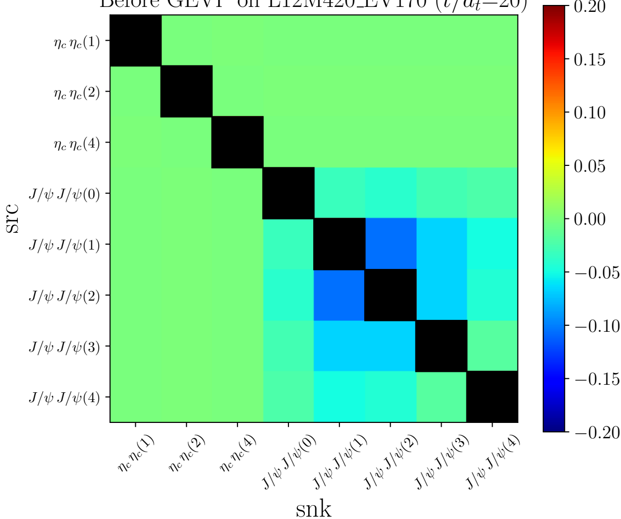
Before GEVP on L12M420_EV170 ( t/a_t=20 )
