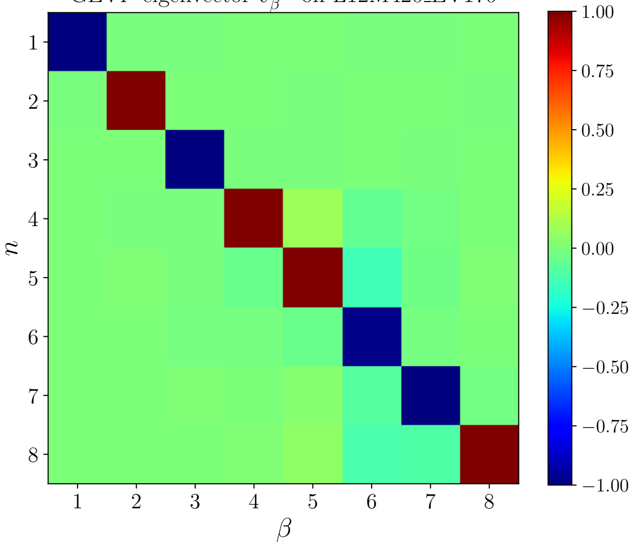
GEVP eigenvector v_{\beta}^{(n)} on L12M420_EV170
