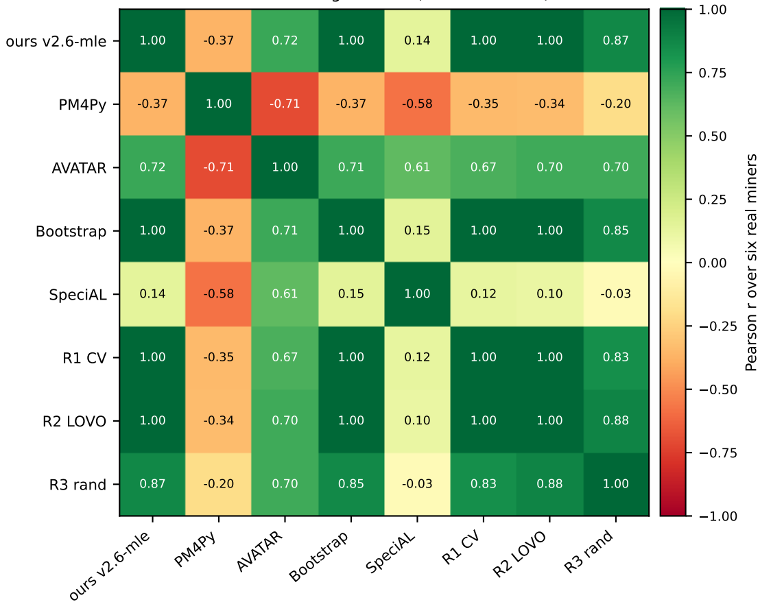
Inter-metric agreement (six real miners)
