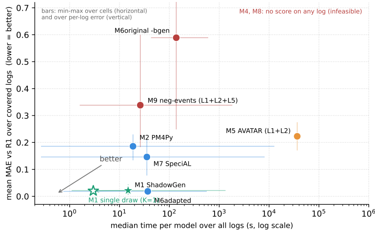
Fig. 6. Speed against accuracy over all five logs: median time per model (log scale) versus mean of the per-log MAEs to R1; lower-left is better. Whiskers show the spread the aggregates hide: horizontal, min to max cell runtime; vertical, min to max per-log MAE. M1 ShadowGen and M6adapted are alone in the accurate corner; M2 PM4Py is fast but never accurate; M9 negative events is fast but poorly calibrated (plotted on the three logs it covers); the Entropia -bgen F-measure (M6original) is slow and the worst-calibrated method that returns; M5 AVATAR is a budget sentinel on all five logs, plotted at its measured GPU training cost (median \sim 10 h per log over L1/L2; the CPU projection is 3–4 days; Sect. 6.2.1) without a time whisker, its accuracy read from the two small logs it scores off-protocol. Partial-coverage points carry their logs in the label. M4 and M8 do not complete a scorable comparison.
