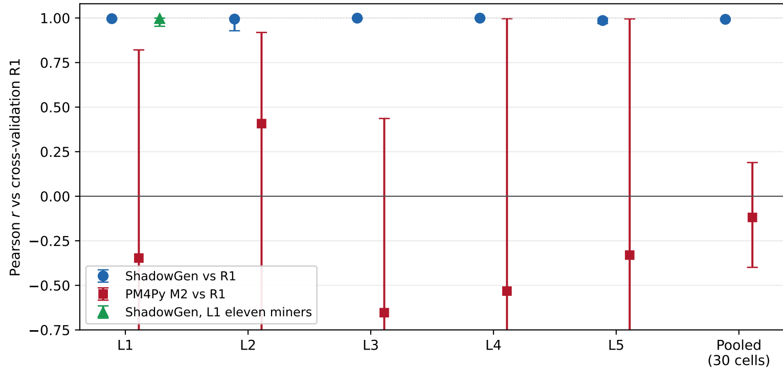
Agreement with the ground truth: bootstrap 95% CIs (ShadowGen tight and high; PM4Py straddles zero)
