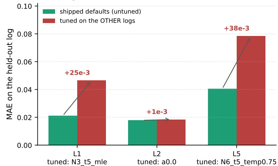
(c) tuning does NOT transfer: it makes it worse
