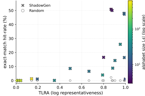
Fig. 5. Generator premise across the 21-log catalog: exact-match hit-rate against log representativeness (TLRA), ShadowGen crosses coloured by alphabet size |A| vs the uniformly random floor (open circles), one point per log. ShadowGen exceeds random on every log (random never above 2.2%). Two structural properties shape exact-matchability: hit-rate correlates with representativeness (Pearson 0.66 with TLRA) and against alphabet size (Pearson -0.65 on \log |A| ). The floor cluster is the large-alphabet municipality logs ( |A| up to 624), which are also the least representative, so both properties push them to zero.
