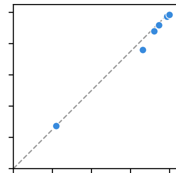
Bootstrap (MAE 0.018)
