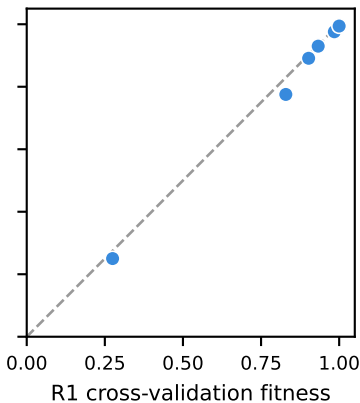
Bootstrap (MAE 0.018)
