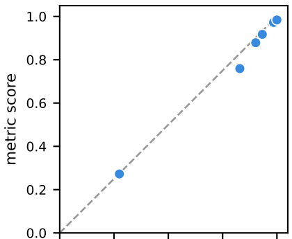
Bootstrap adapted (MAE 0.018)
