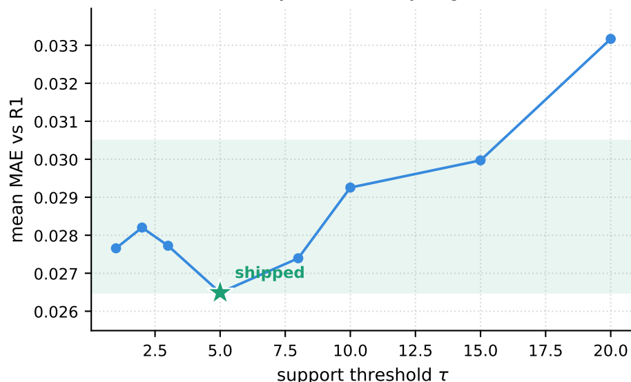
\tau : shallow basin; only \tau \geq 10 clearly degrades
