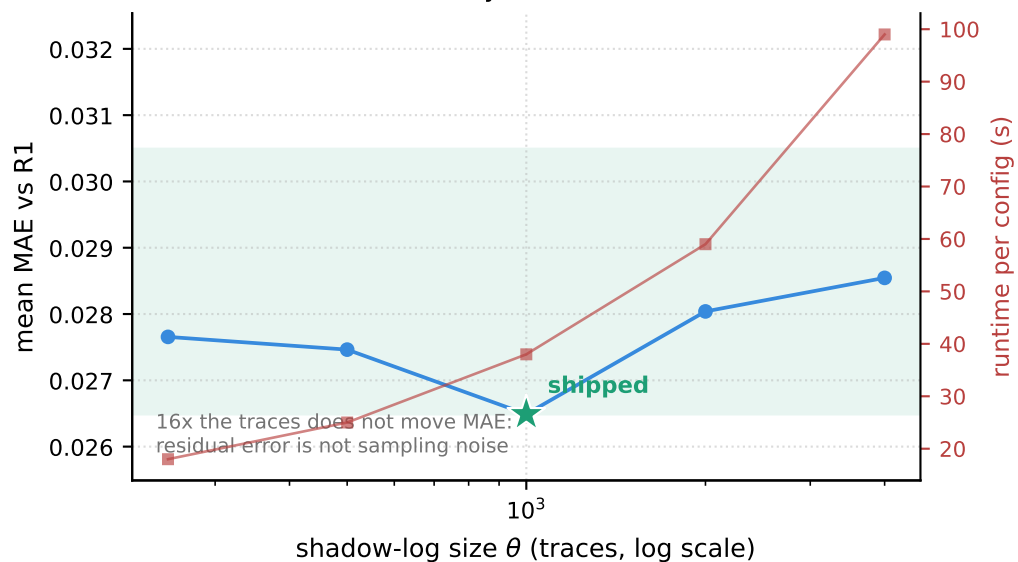
\theta : inert. the error floor is systematic
