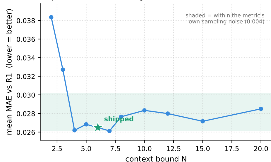
N: plateau from 4, nothing above 8
