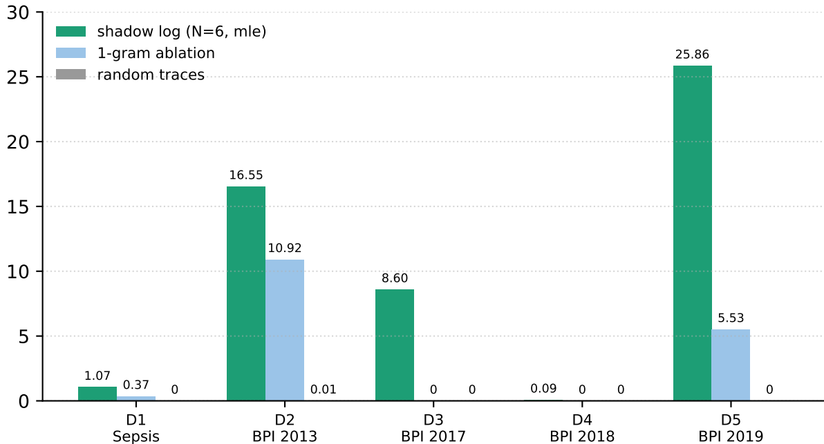
% of generated traces that are held-out REAL variants
