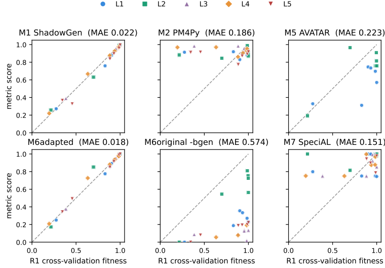
Fig. 7. Per-method calibration against the cross-validation ground truth R1 across all five logs (six non-degenerate miners per log, up to 30 points, one marker per log; dashed line y=x ). The generative and resampling metrics (M1 ShadowGen, M6adapted) sit on the line on every log; the published Entropia -bgen F-measure of the same bootstrap sample (M6original) sits far below it (its F1 folds precision in, Sect. 6.2.3); M2 PM4Py forms a flat band that ignores the ground-truth gradient; M5 AVATAR (shown off-protocol on L1/L2 only, Sect. 6.2.1) and M7 Special scatter off the line. Metrics that could not run on every log appear with fewer points: AVATAR’s sparse panel is itself the feasibility verdict.
