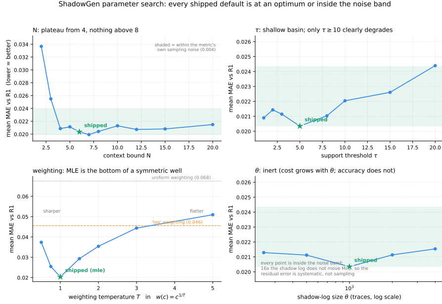
Fig. 11. One-factor sweeps around the shipped configuration (star): MAE to R1 over the six non-degenerate miners of all five logs at K=1 ; the shaded band is the metric's own sampling variance (0.004). N plateaus from 4 out to 20. \tau is a shallow basin with its minimum at the shipped 5. The weighting is a symmetric well with MLE at the bottom; the log alternative and uniform weighting cost roughly twice and three times the calibration error. \theta is flat while its cost grows linearly, so the residual error is systematic, not sampling noise.
