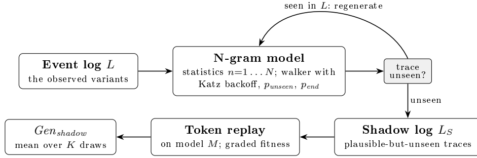
Fig. 3. ShadowGen pipeline. From the variants of the event log L , N-gram statistics up to order N feed a stochastic walker (Katz backoff; novelty probability p_{\text{unseen}} ; termination probability p_{\text{end}} ). A generated trace that copies an observed variant is regenerated, so the shadow log L_S contains only unseen traces. The model M under evaluation enters only at the replay step, which yields the metric: the graded score Gen_{\text{shadow}} , averaged over K draws. A strict acceptance reading of the same shadow log ( Gen_{\text{accept}} ) exists as a validation diagnostic (Sect. 6.2.5), not as part of the released metric.
