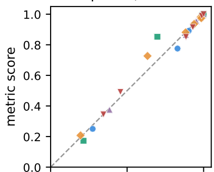
M6adapted (MAE 0.018)
