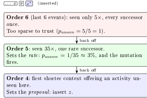
Fig. 10. Katz-consistent mutation at realistic counts (illustrative; activities abstracted to x, y, z ). Backoff sets both how often to invent an event (the rate, resolved at order 5) and what to invent (the proposal, found at order 4): novel in the exact context, yet attested in a related shorter one.
