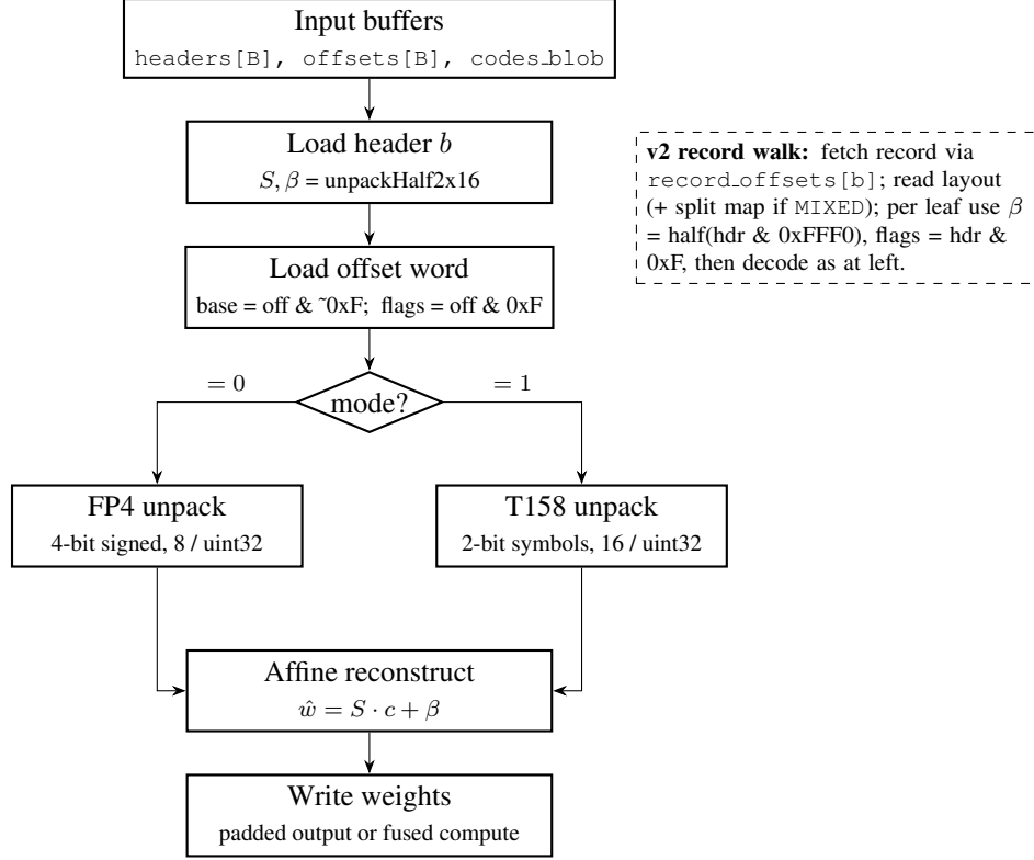
Figure 4: GPU unpack and affine reconstruction flow (v1 path shown; dashed note gives the v2 record walk).
