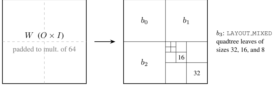
Figure 1: Tiling a weight matrix into 64 \times 64 macroblocks. In the v1 profile every macroblock is one block. In the v2 profile a macroblock may be subdivided by an error-driven quadtree ( b_3 shown); each leaf carries its own scale, bias, and code mode.
