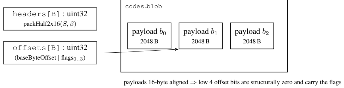
Figure 2: v1 container: two parallel metadata arrays index a blob of constant 2048-byte payloads. Headers supply affine parameters; aligned offsets carry the mode flag at zero metadata cost.
