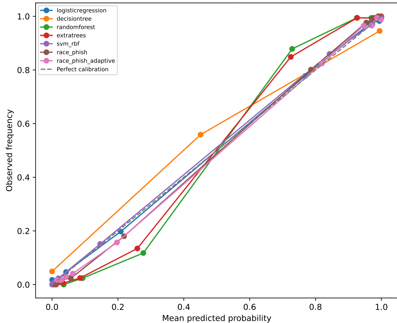
Calibration Comparison
