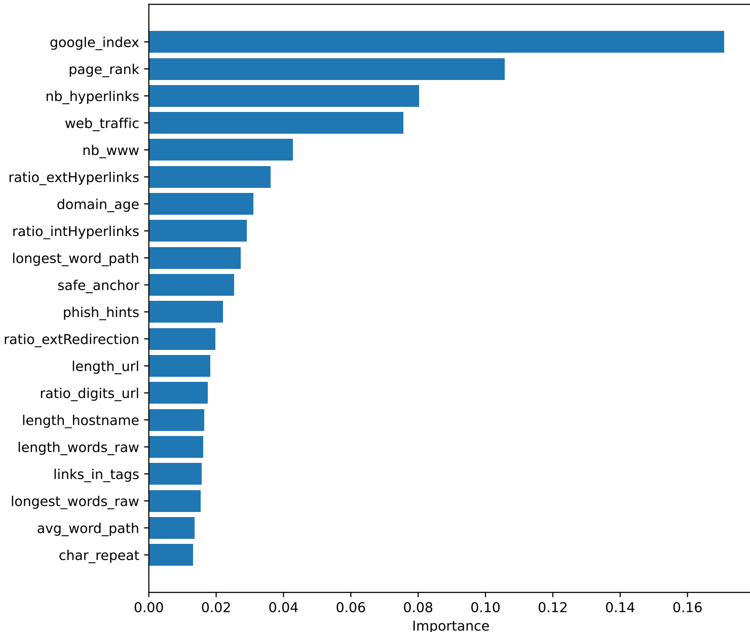
Top 20 Feature Importance (Random Forest)
