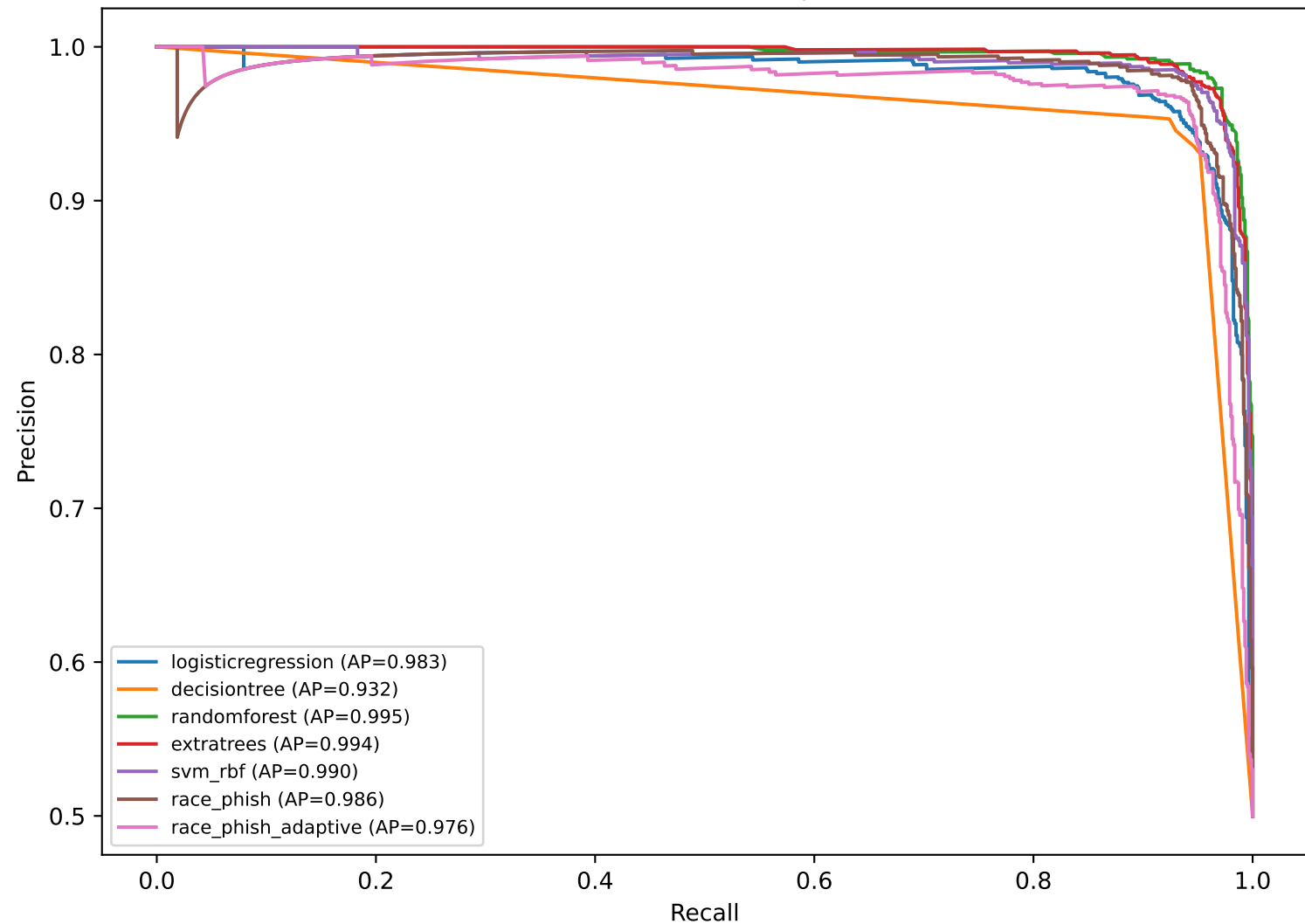
Precision-Recall Comparison
