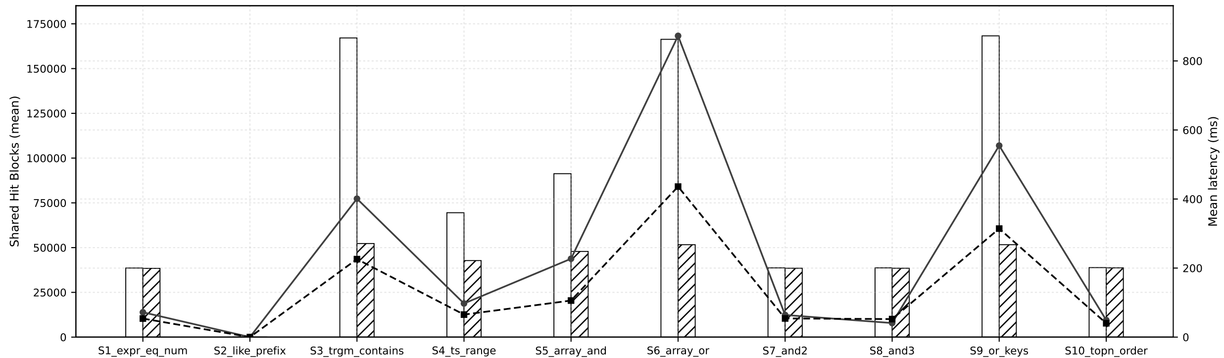
Shared Hits (bars) + Mean latency (lines) — Indexed JSONB vs REL — N=1,000,000
