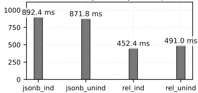
S8 — Multi-key AND (3 keys)
