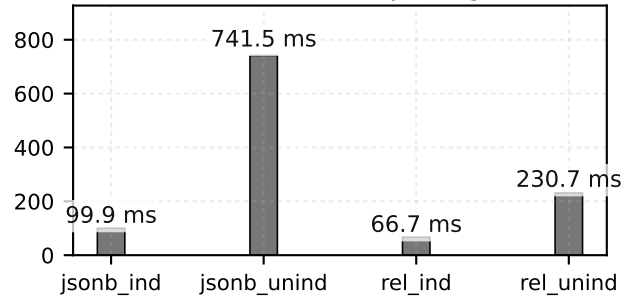
S6 — Array OR (any overlap)
