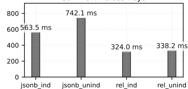
S9 — OR Across Keys
