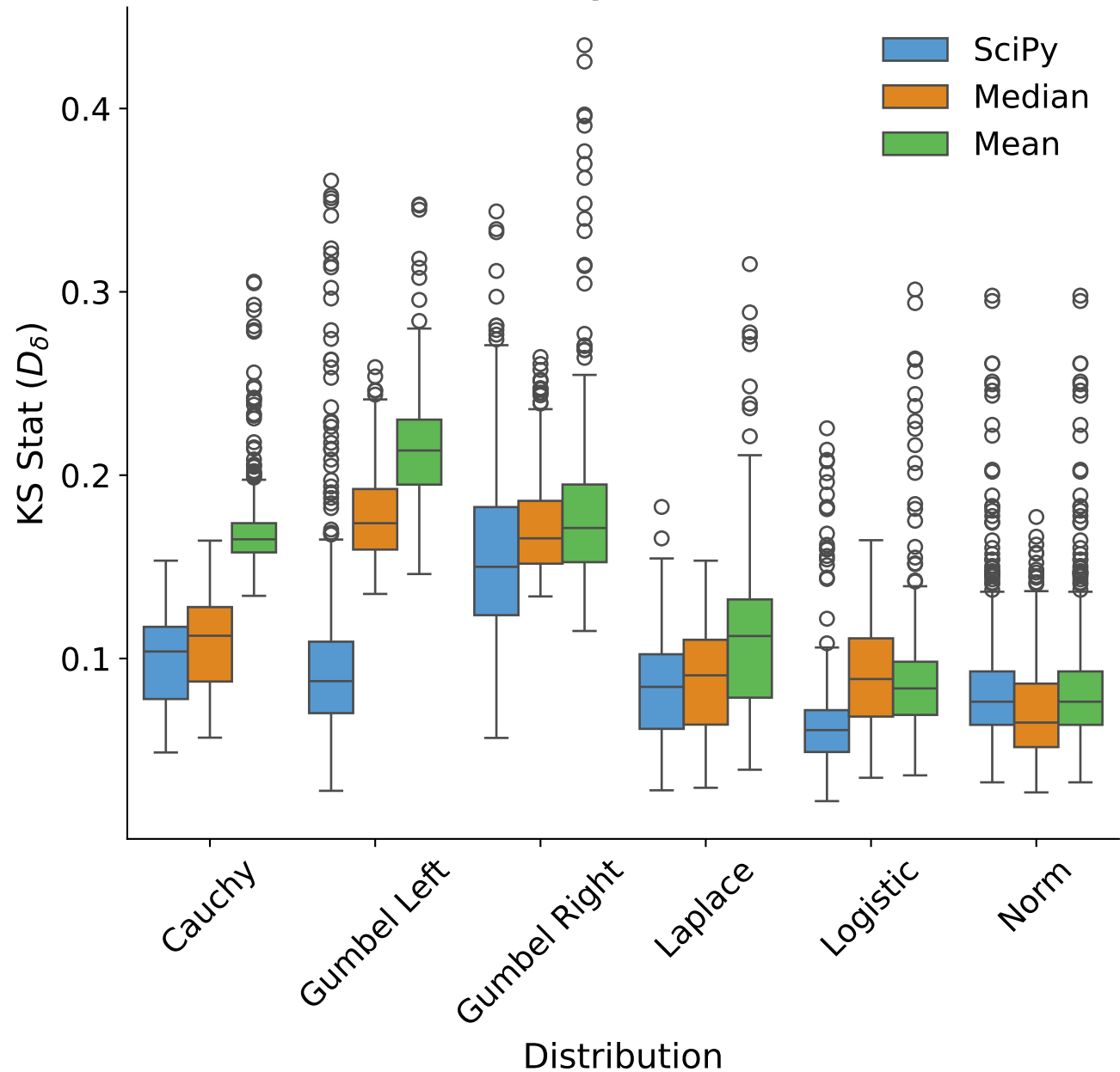
KS Statistic per Distribution
