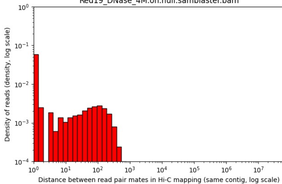
Mate distance distribution for first 3939215 read pairs for sample Red19_DNase_4M.on.null.samblaster.bam
