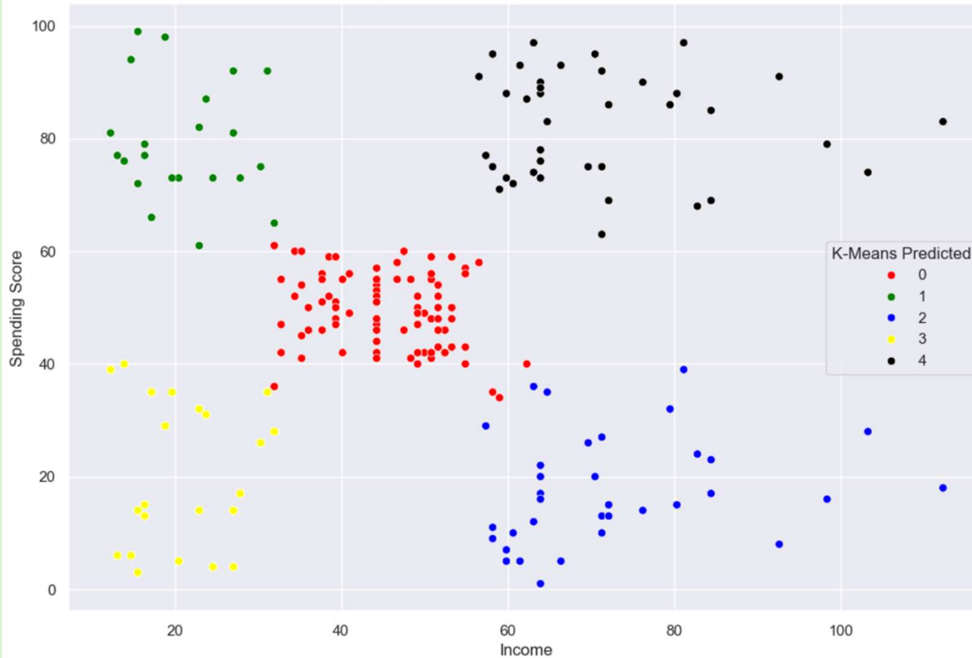
Scatterplot showing spending score compared to income showing K-Means clusters
