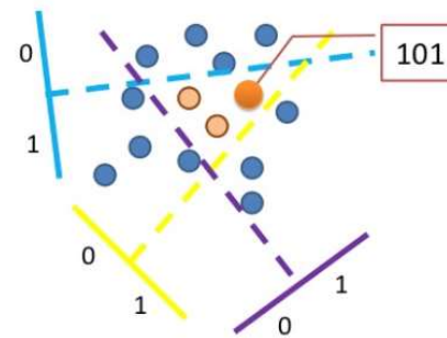
Binary Locality Sensitive Hashing
