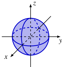
2-norm
