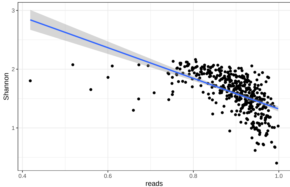
Sequencing depth vs. Shannon – global
