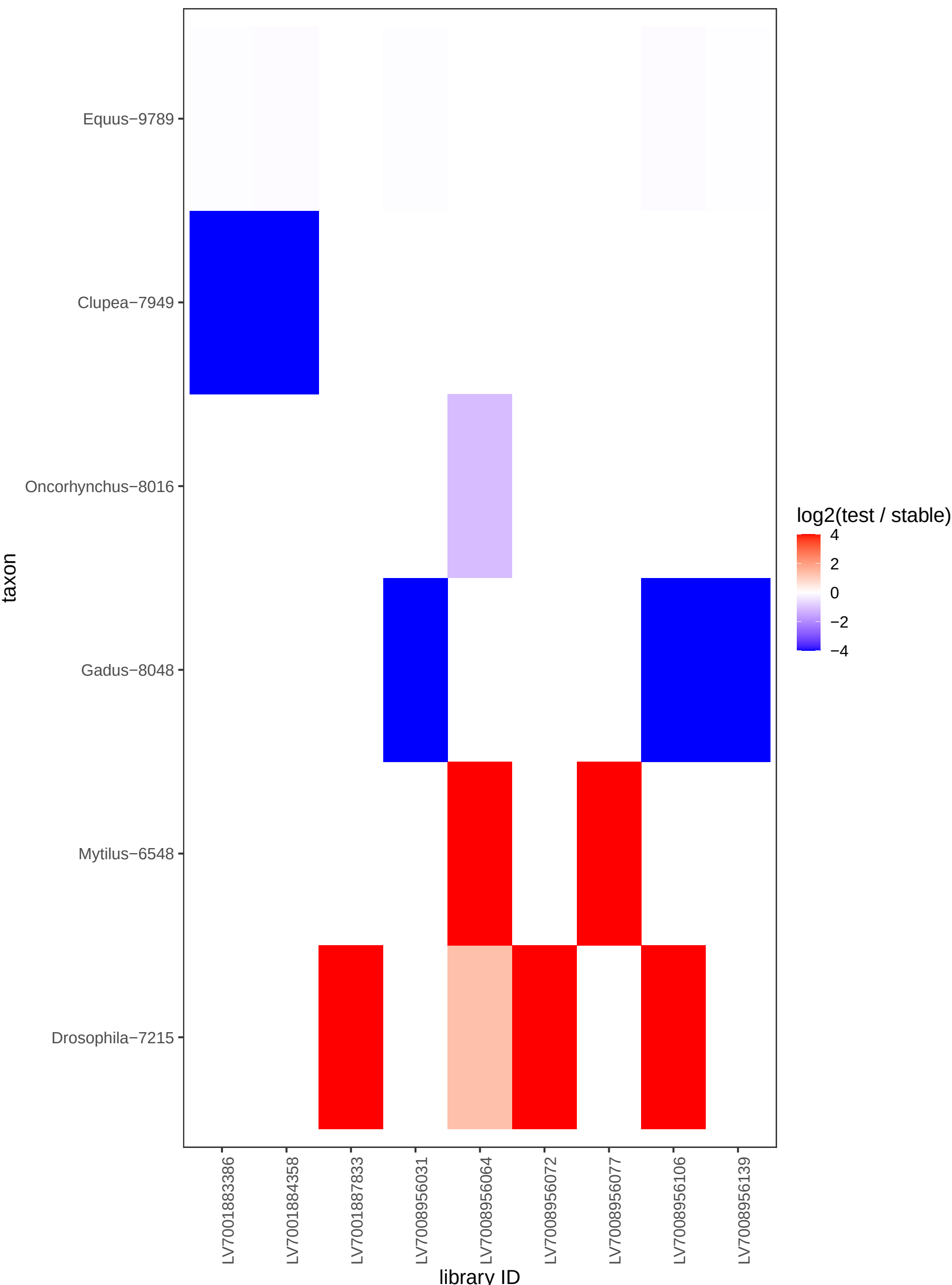
Log2 ratio heatmap (test vs stable) dataset: Tjornen | Group: animal
