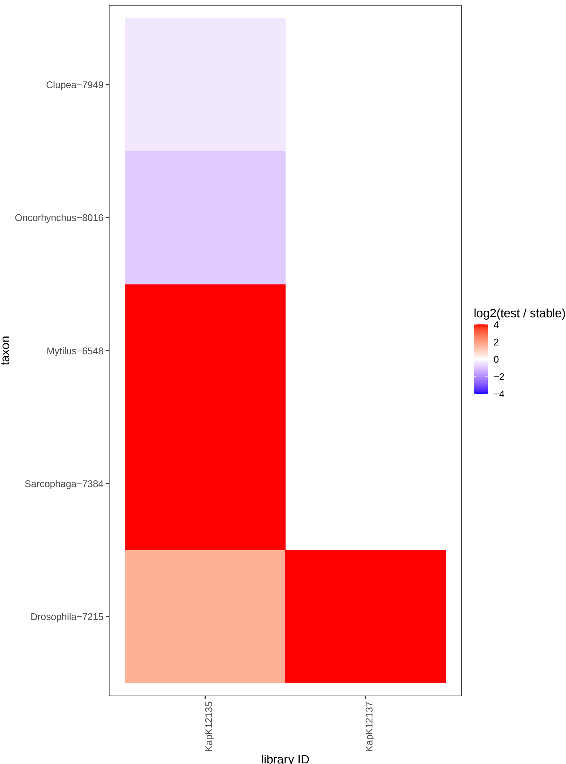
Log2 ratio heatmap (test vs stable) dataset: KapKBH | Group: animal
