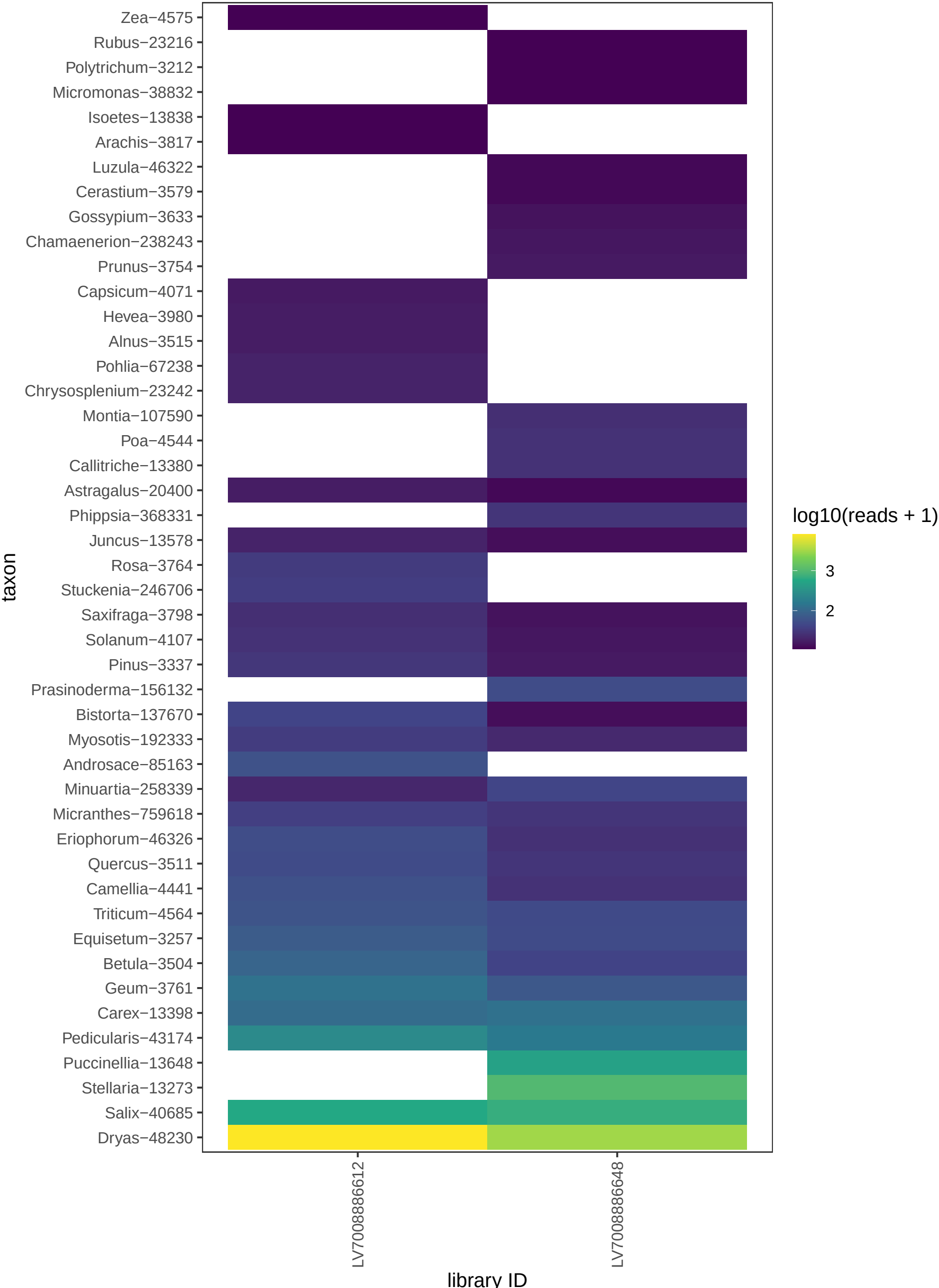
stable – Top 100 Genera in Ellesmere ( plant )
