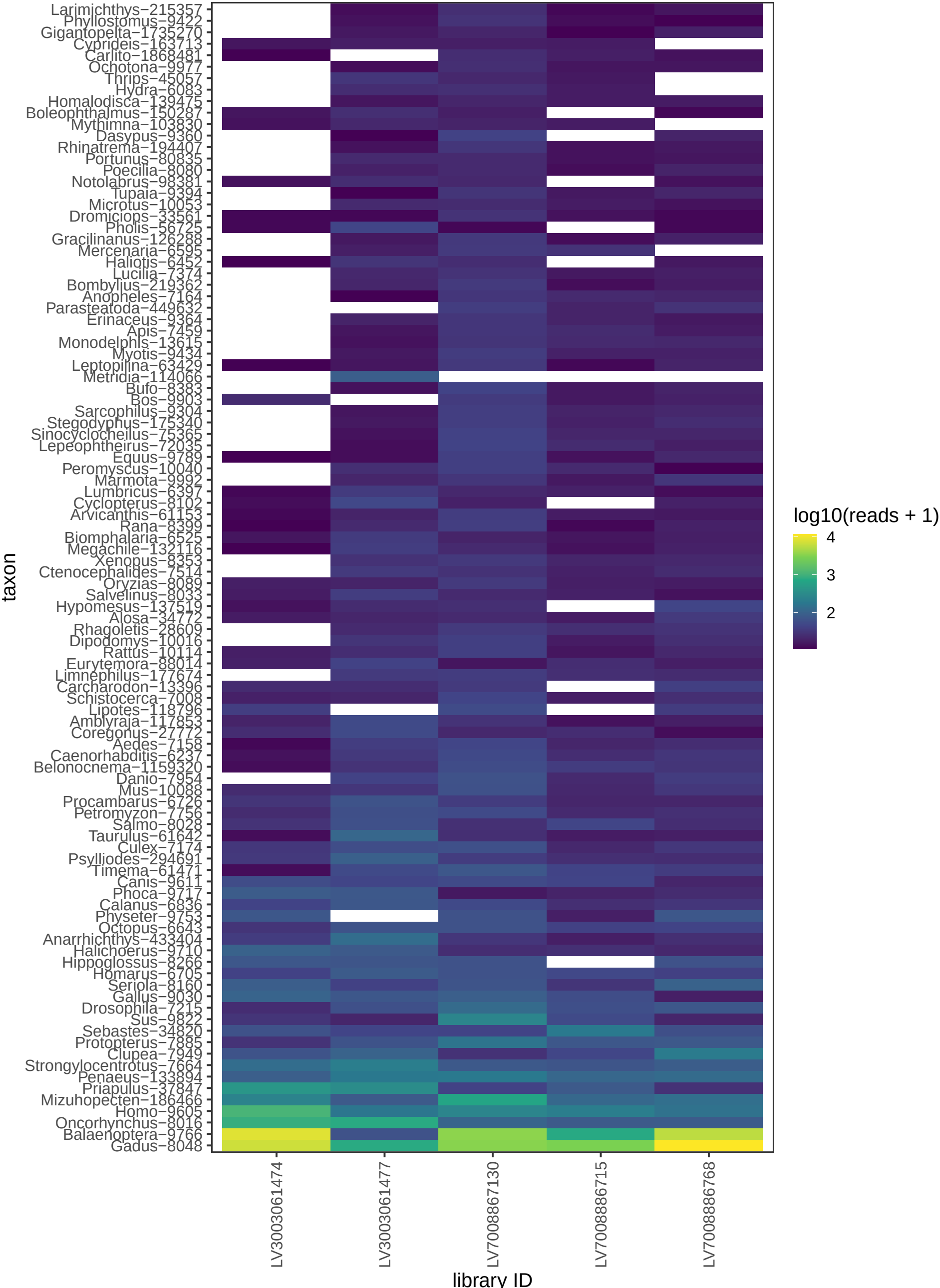
stable – Top 100 Genera in ROCS ( animal )
