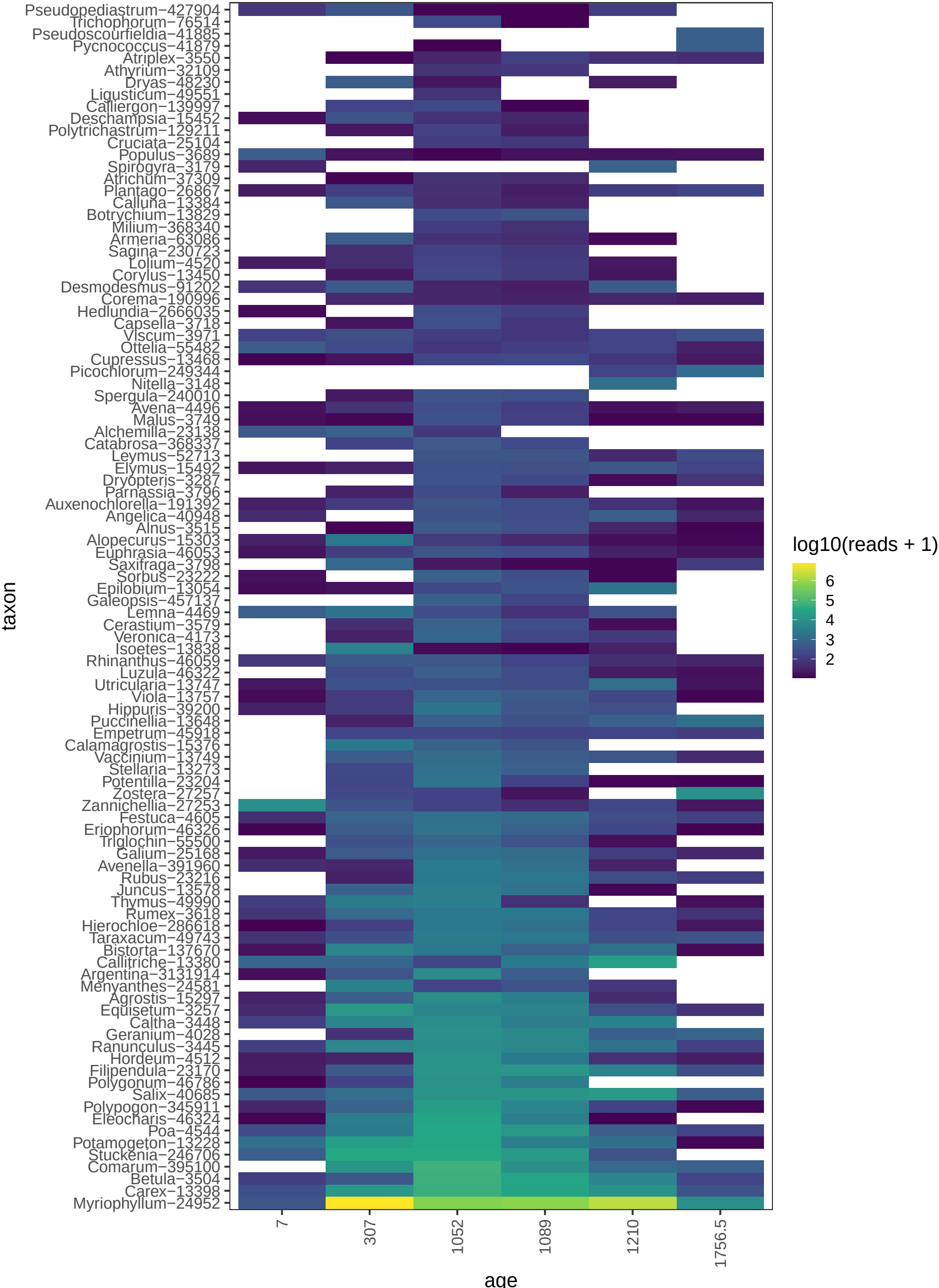
test – Top 100 Genera in Tjornen ( plant )
