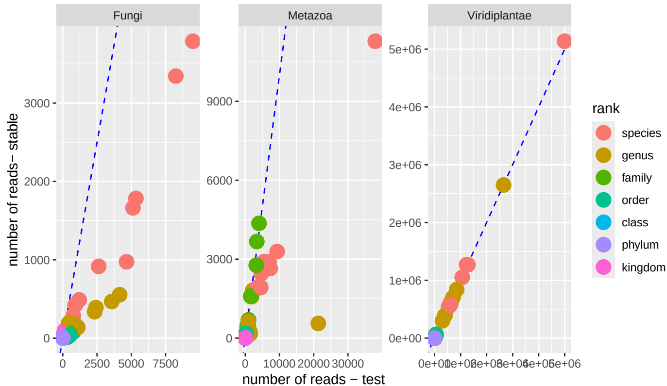
Number of reads per rank in Tjornen
