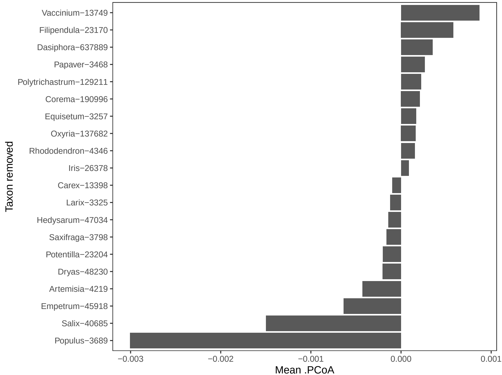
PCoA influencers | Label: KapKBH | Group: plant
