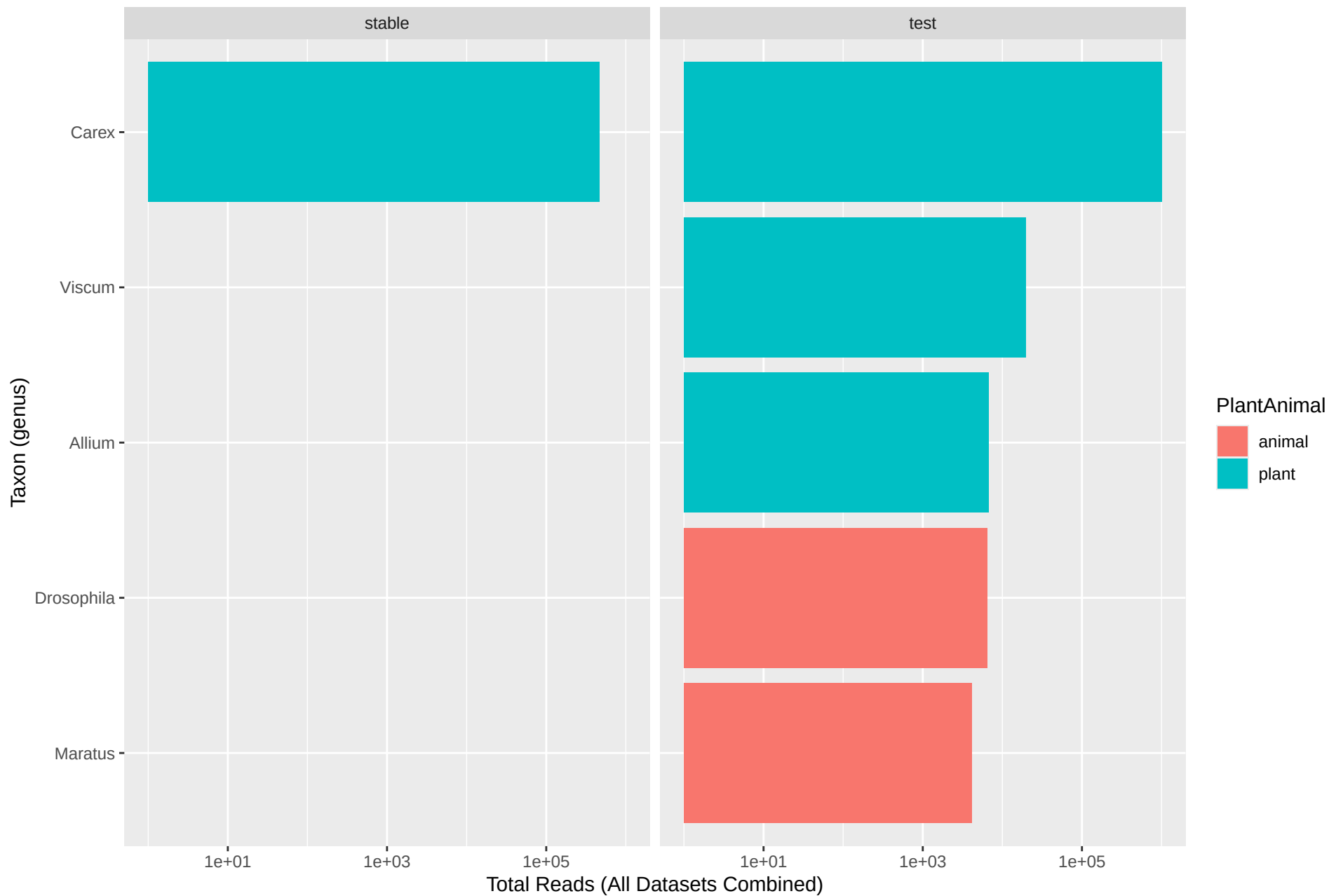
Taxa Found in All Datasets ( \geq 100 reads)
