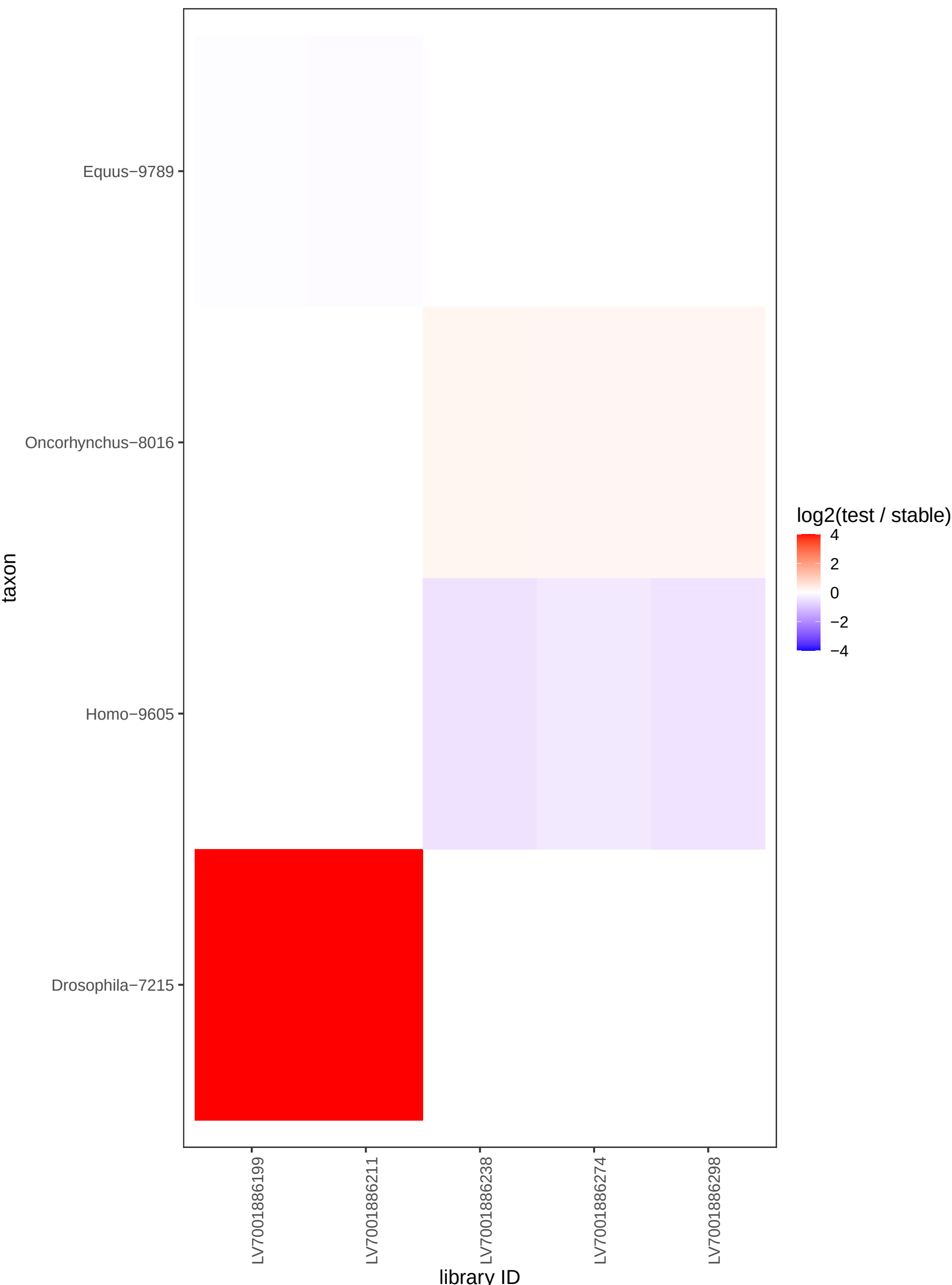
Log2 ratio heatmap (test vs stable) dataset: Yana | Group: animal
