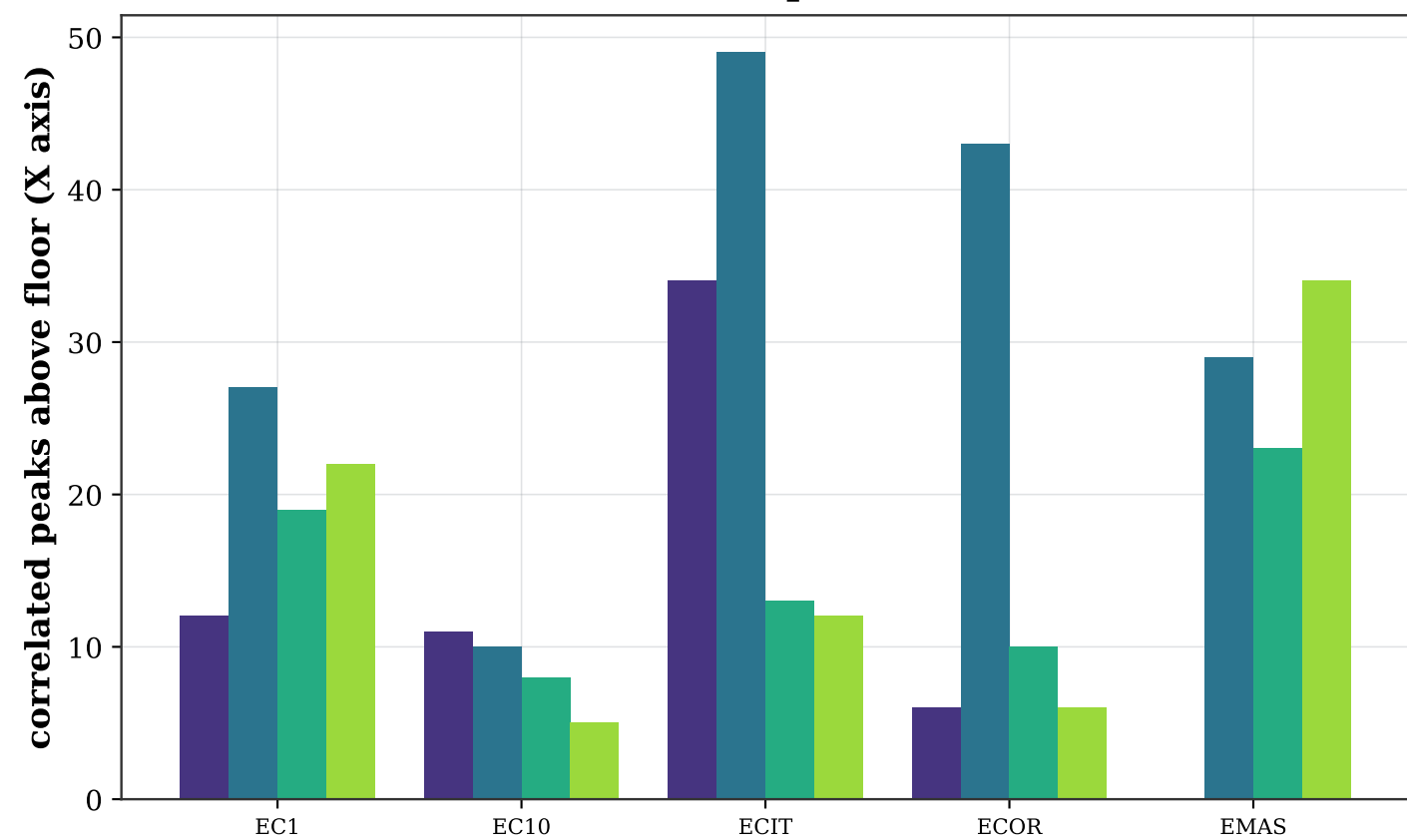
IMPROVE (quiescent)
