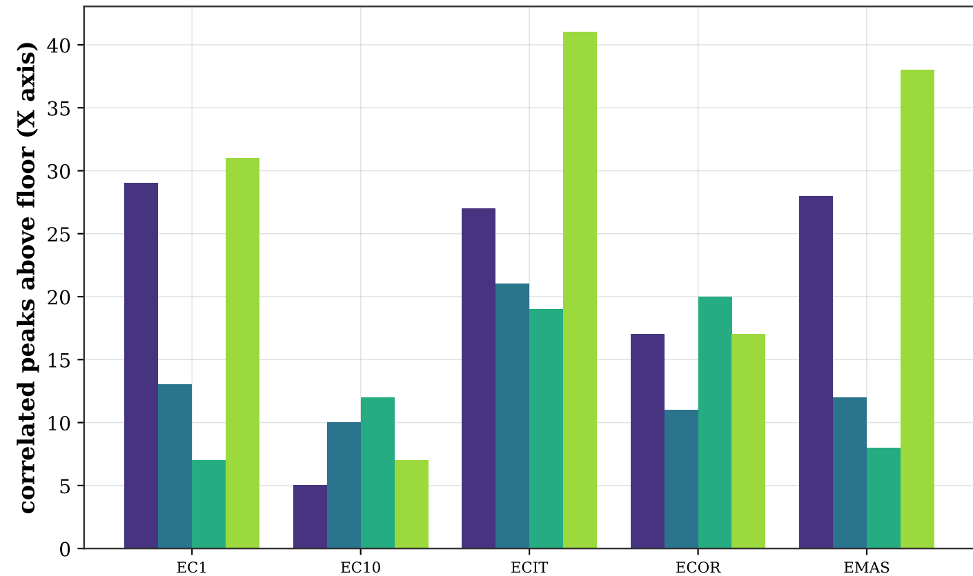
IMPROVE (quiescent)
