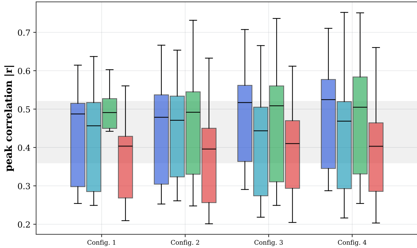
IMPROVE (quiescent)
