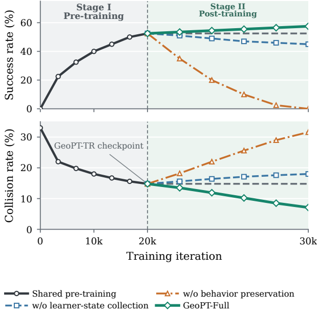
Fig. 7. Two-stage training dynamics. Success rate (top) and collision rate (bottom) across shared behavior-prior initialization and privileged post-training.
