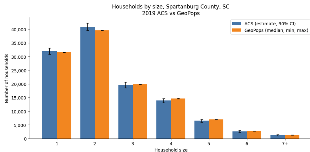
Figure 1: Comparison of ACS and GeoPops for number of households by household size for Spartanburg County, SC. Ninety percent confidence intervals (CI) for ACS data (blue) are calculated using margin of error values provided by the US Census (United States Census Bureau, 2019). GeoPops data (orange) include the median with minimum and maximum range from 100 population synthesis runs. The ranges for household size counts resulting from 100 GeoPops runs fall within the 90% CI ACS estimates, except for 2-person households where the GeoPops maximum overlaps with the ACS lower bound by ~50 households.
