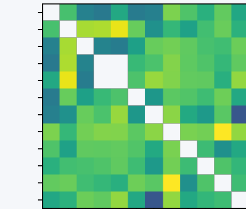
Correlation
