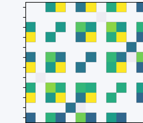
Hsim_Distance
