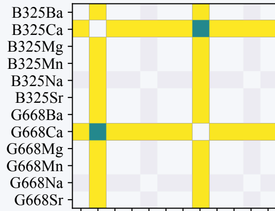
Euclidean
