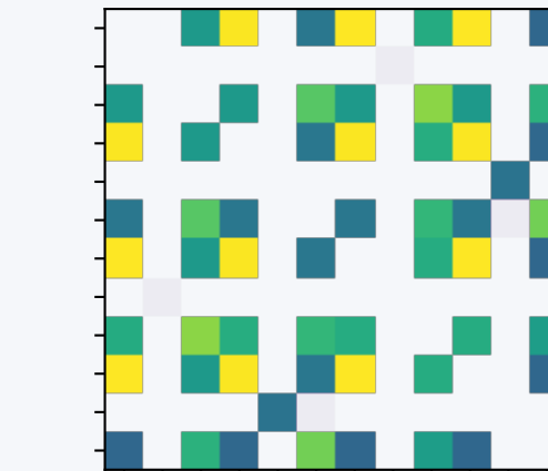
Close_Distance
